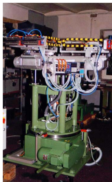
Abb. 3: Handlingsystem
